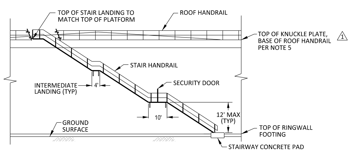
STAIR ELEVATION
