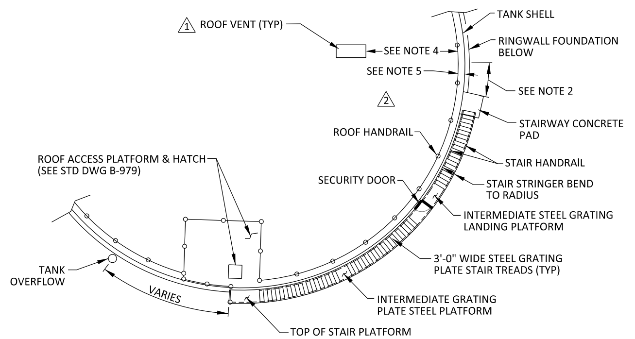
EXTERIOR STAIR PLAN
