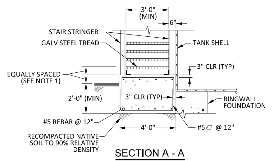
STAIRWAY HANDRAIL AND CONCRETE PAD
